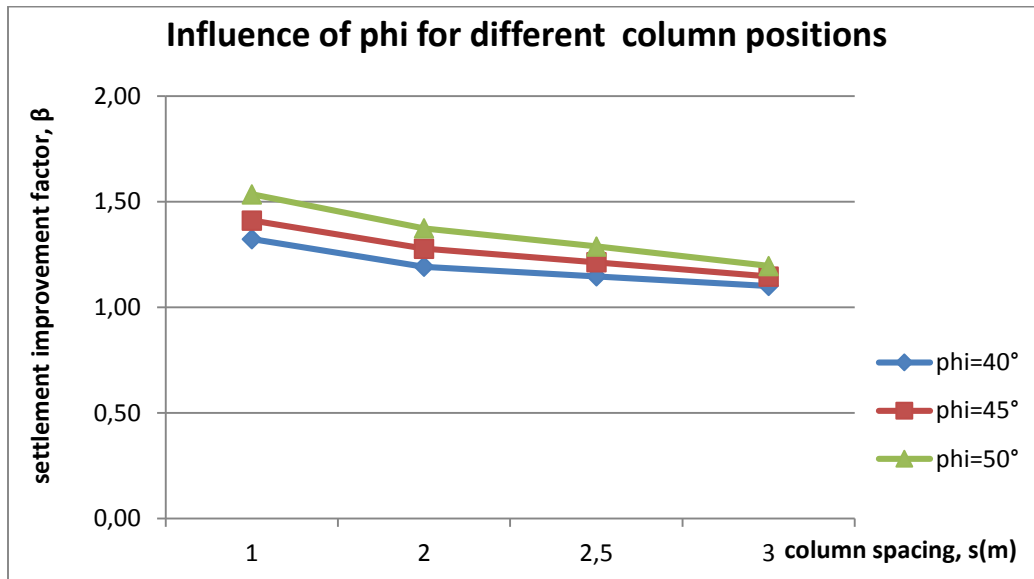
Fig. 6. The effects of the Internal friction angle of columns and their spacing.
