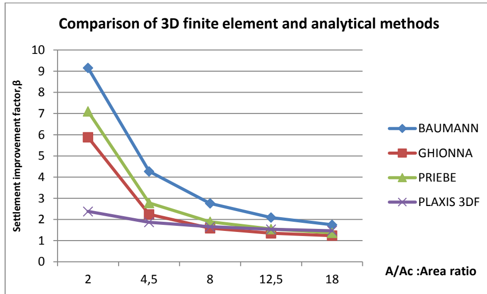
Fig. 2. Comparison of Numerical modeling (Plaxis 3DF) and analytical methods.
