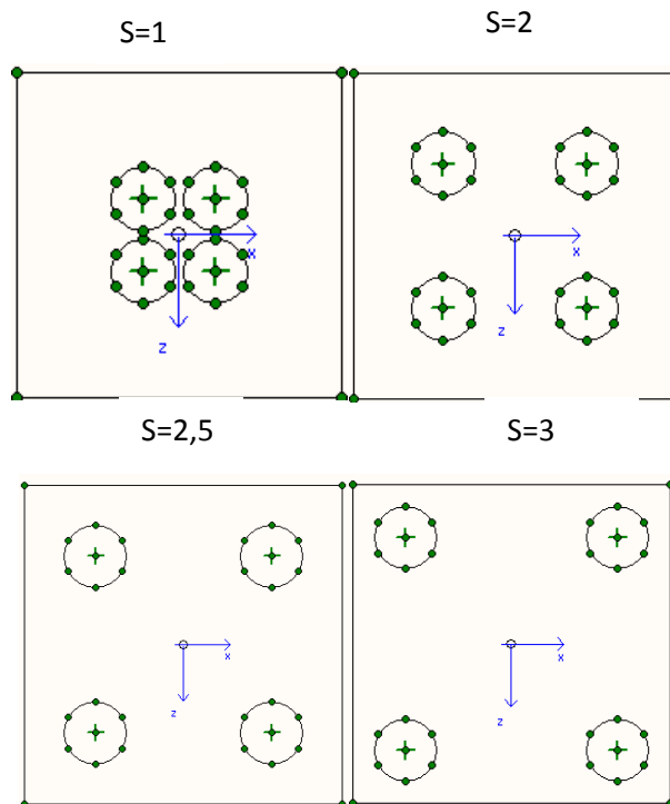
Fig. 3. The Variation of the columns spacing for a rectangular mesh
