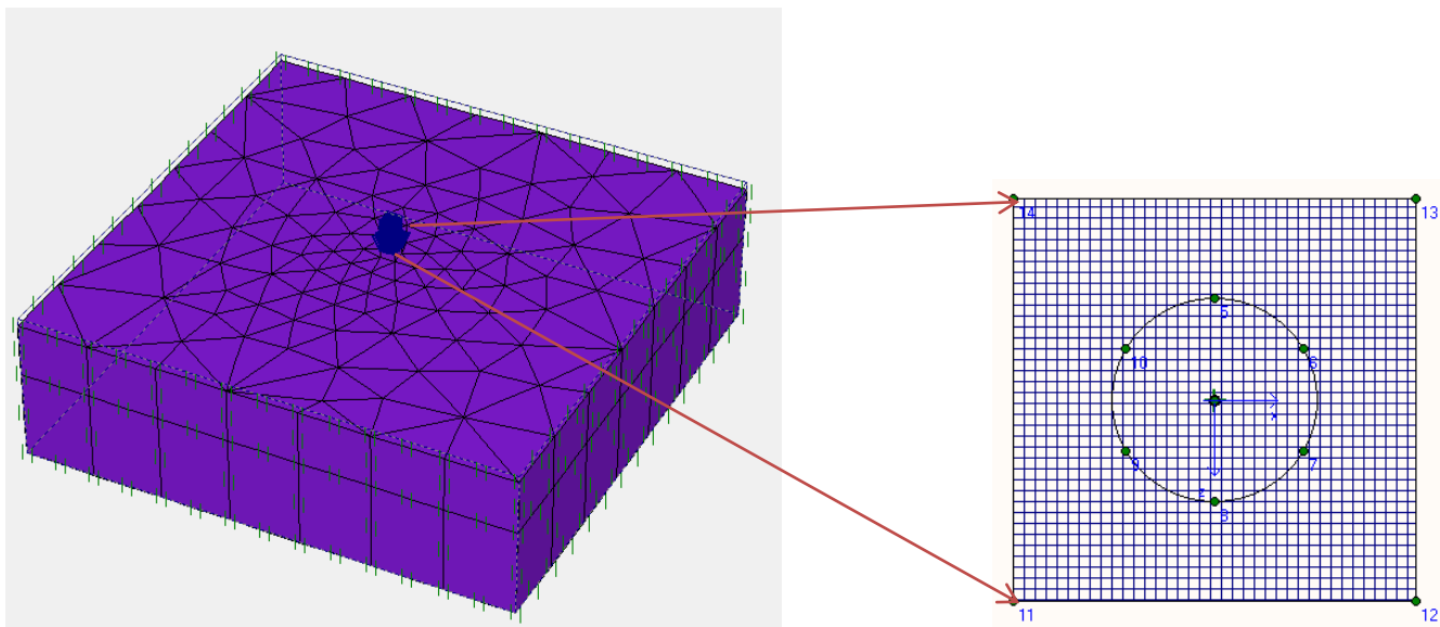
Fig. 1. Numerical modeling (Plaxis 3DF) of an isolated stone column.
