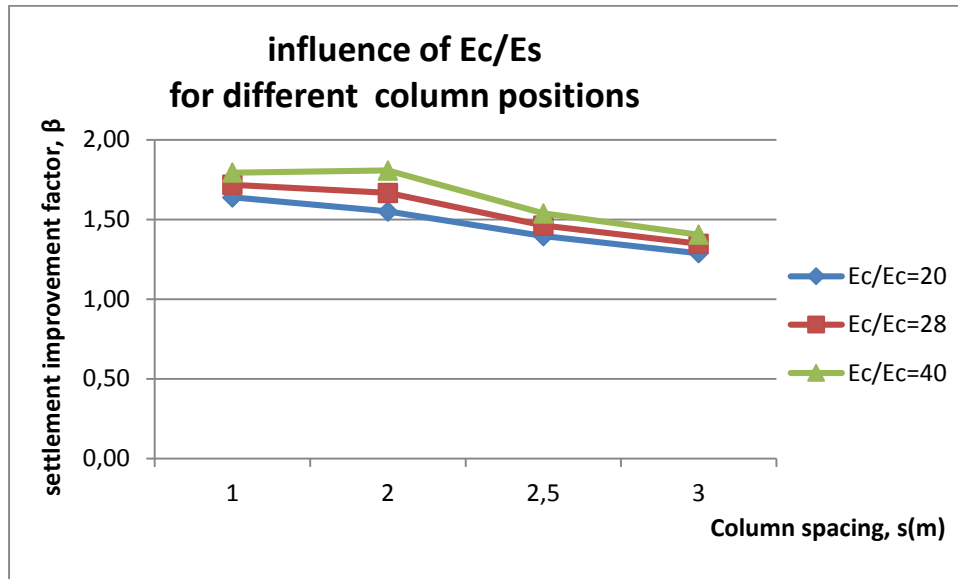
Fig. 7. The effects of The columns modular ratio and their spacing.
