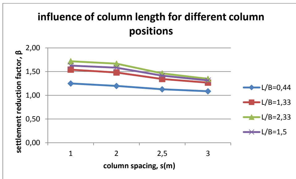
Fig. 8. Influence of column length for different column positions.
