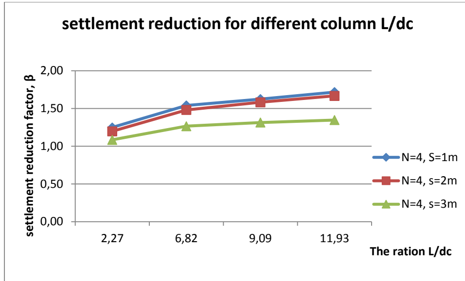
Fig. 9.settlement reduction for different column L/dc.
