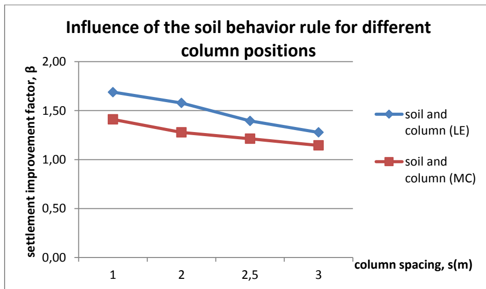
Fig. 5. The effects of the soil behavior rule and the columns spacing.
