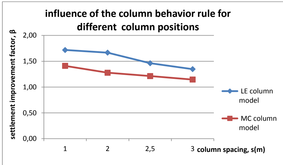
Fig. 4. The effects of the columns behavior rule and their spacing.
